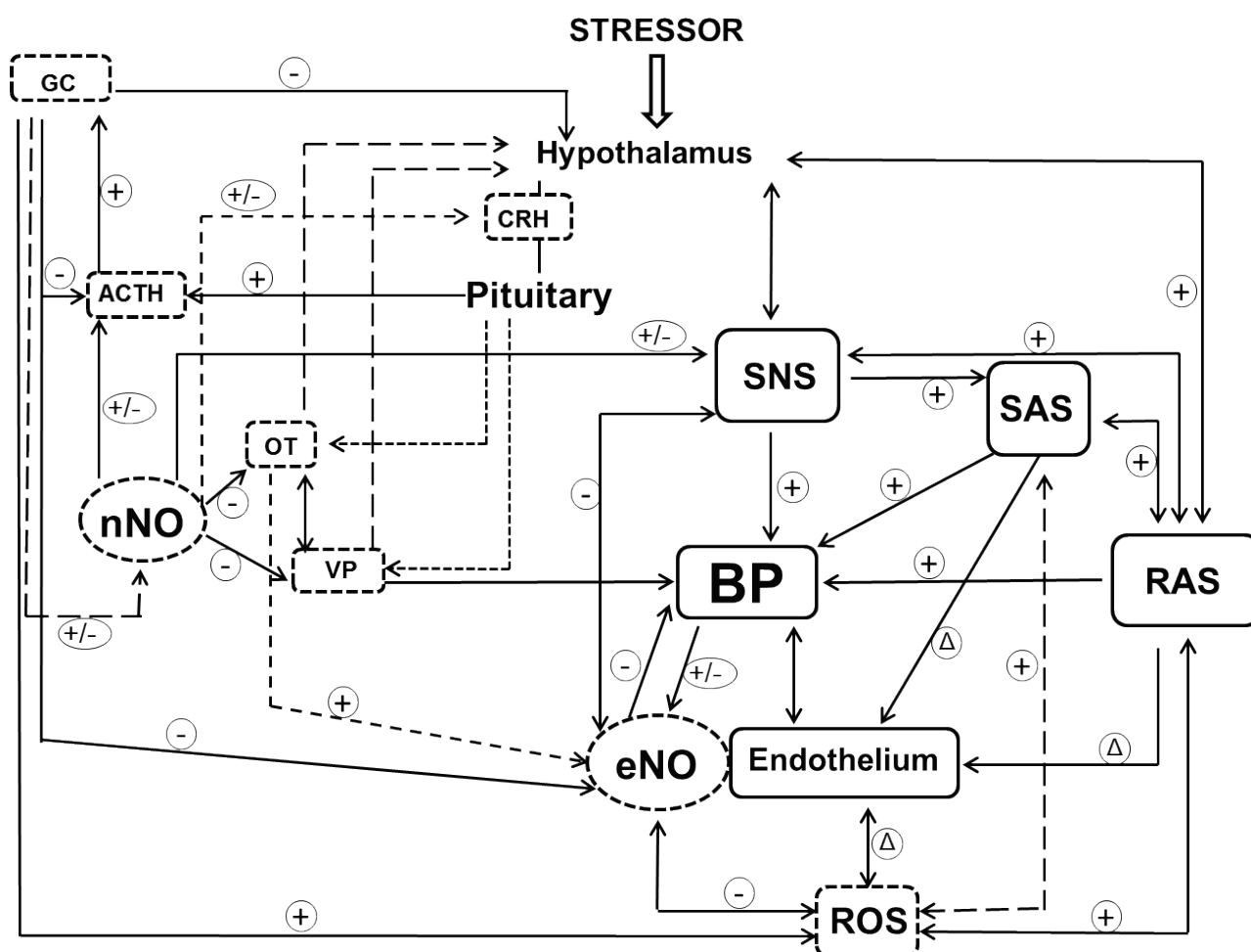
Fig. 2. A simplified scheme of nitric oxide involvement in the main blood pressure regulatory mechanisms in stress. Inhibiting effects are marked by "minus" mark, activating effects are marked by "plus" mark. The alterations in endothelial function (including those other than NO-mediated) are marked by \Delta . ACTH – adrenocorticotrophic hormone, BP – blood pressure, CRH – corticotropin releasing hormone, eNO – nitric oxide synthesized by endothelial nitric oxide synthase, GC – glucocorticoids, nNO – nitric oxide synthesized by neuronal nitric oxide synthase, NO – nitric oxide, OT – oxytocin, RAS – renin-angiotensin system, ROS – reactive oxygen species, SAS – sympathoadrenomedullary system, SNS – sympathetic nervous system, VP – vasopressin.
